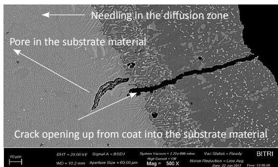
Fig. 4. Sectioned tip
