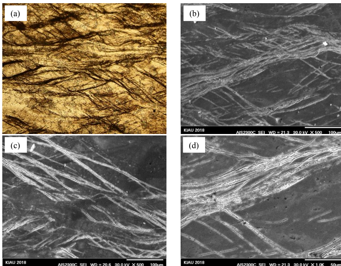
Fig. 3. microstructures of the annealed alloys (a) optical microscopy at 400°C, (b) SEM at 400°C, (c) SEM at 500°C, (d) SEM at 600°C.
