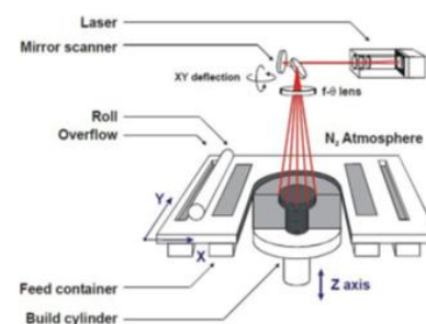
Fig. 2. Schematic representation of an SLM machine [1]
