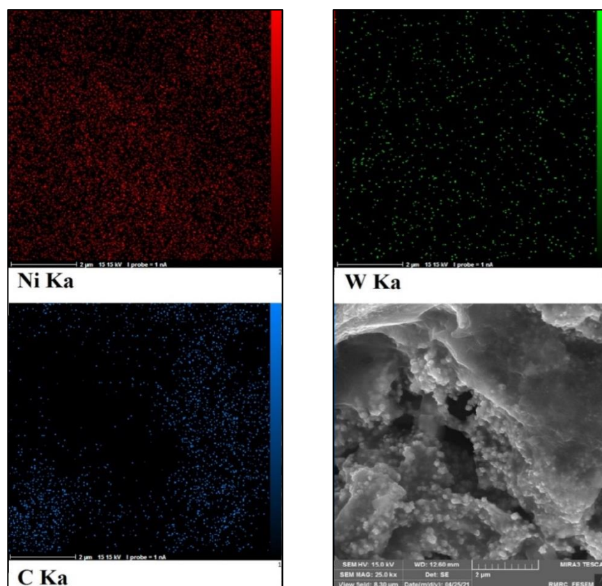
Fig. 3. The results of EDS analysis and dispersion of Ni, W and C elements
