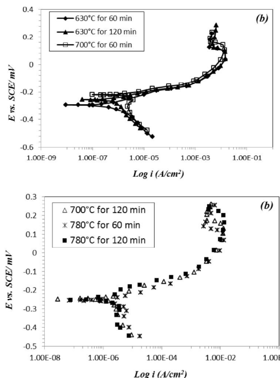
Fig. 4. Polarization curves of the alloys in 3.5% NaCl solution after different annealing temperatures and times: (a) ADB, (b) ALB.
